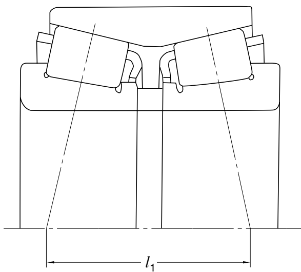
Fig. 1-14 Back-to-Back Arrangement
