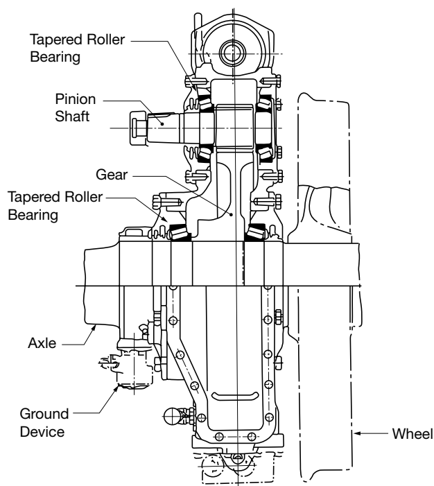
Fig. 3-9 Cardan Drive System with Gear Coupling
