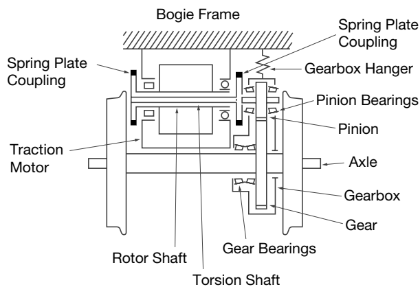
Fig. 3-2 Cardan Drive System with Hollow Shaft Motor
