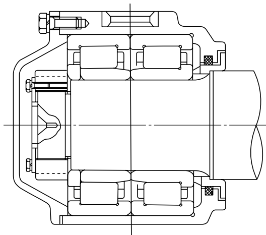
Fig. 1-11 Axle Box with Roller-Guiding Ribs to Sustain Axial Loads (UIC Standard Type)
