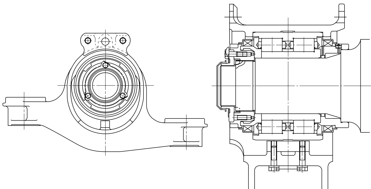
JR East Company, Commuter Train, Series 205 Bearing Number: JC32
