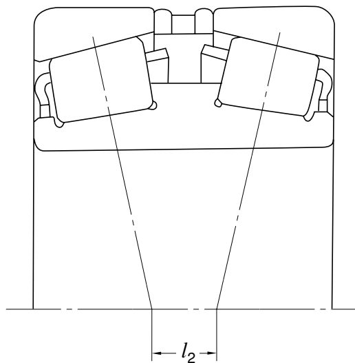
Fig. 1-15 Face-to-Face Arrangement
