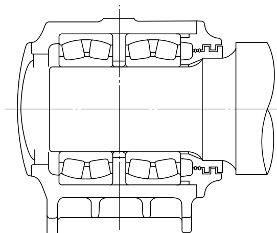
Fig. 1-7 Double Spherical Roller Bearings
