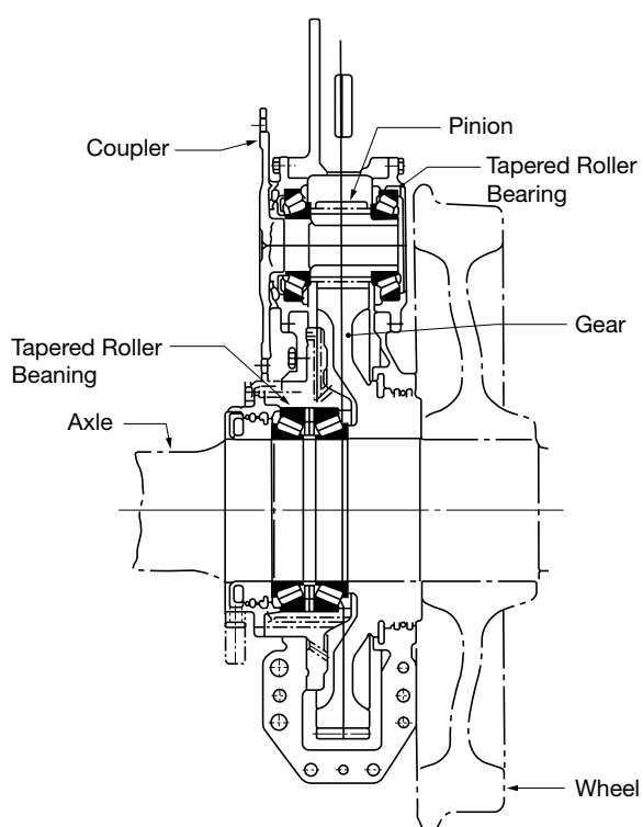
Fig. 3-8 Cardan Drive System with Hollow Shaft Motor
