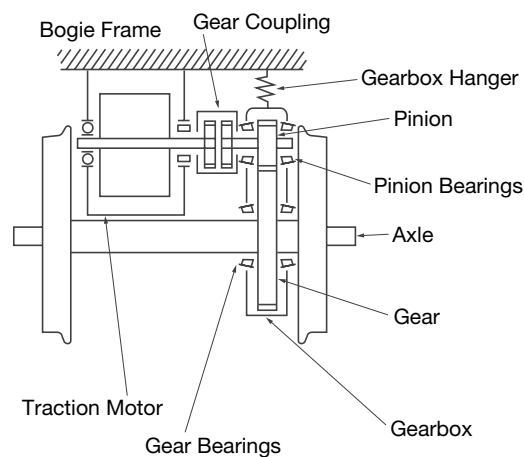
Fig. 3-4 Gear Coupling Drive System
